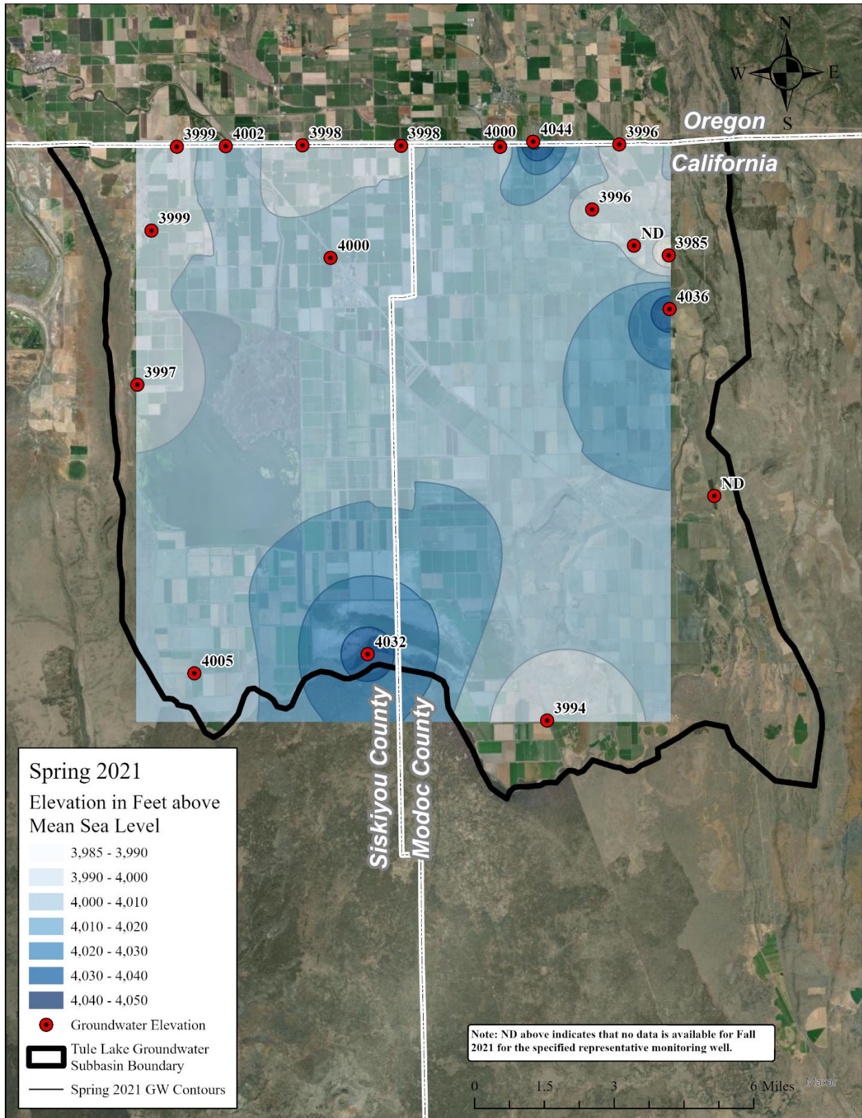
Figure 2-8. Spring 2021 Groundwater Surface Elevations
