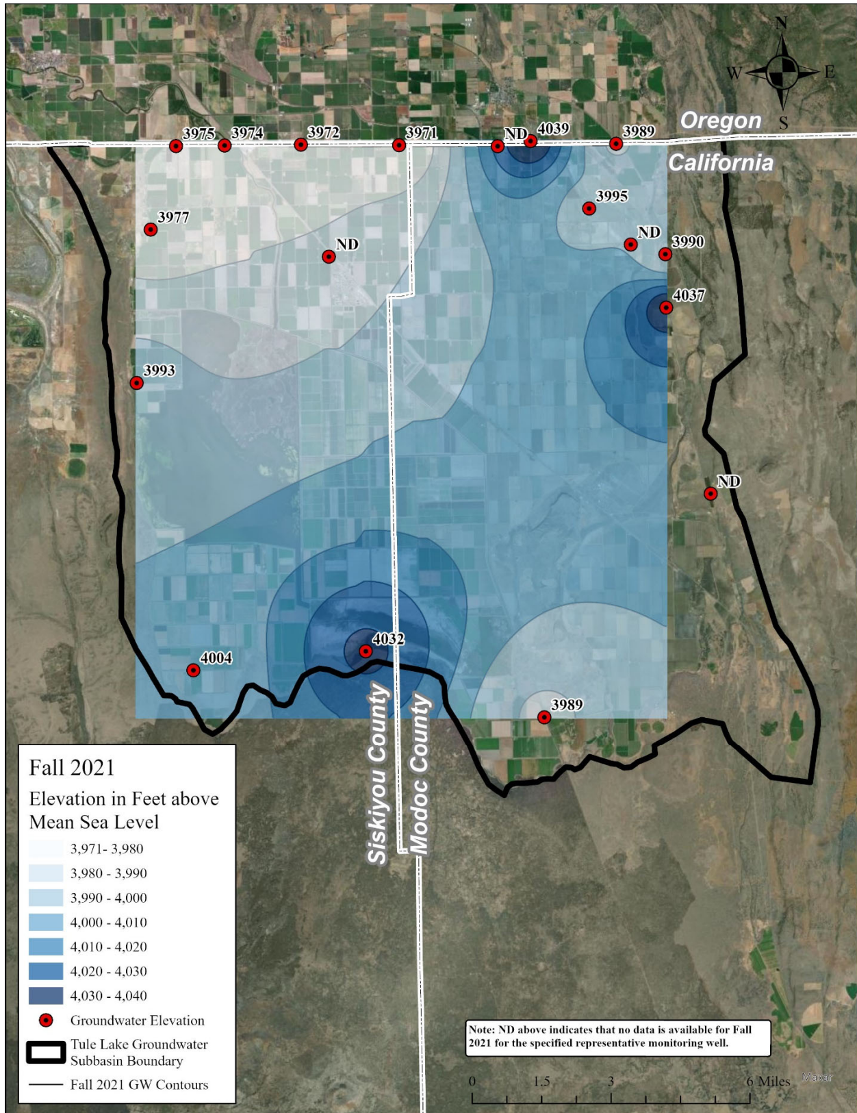
Figure 2-8. Fall 2021 Groundwater Surface Elevations
