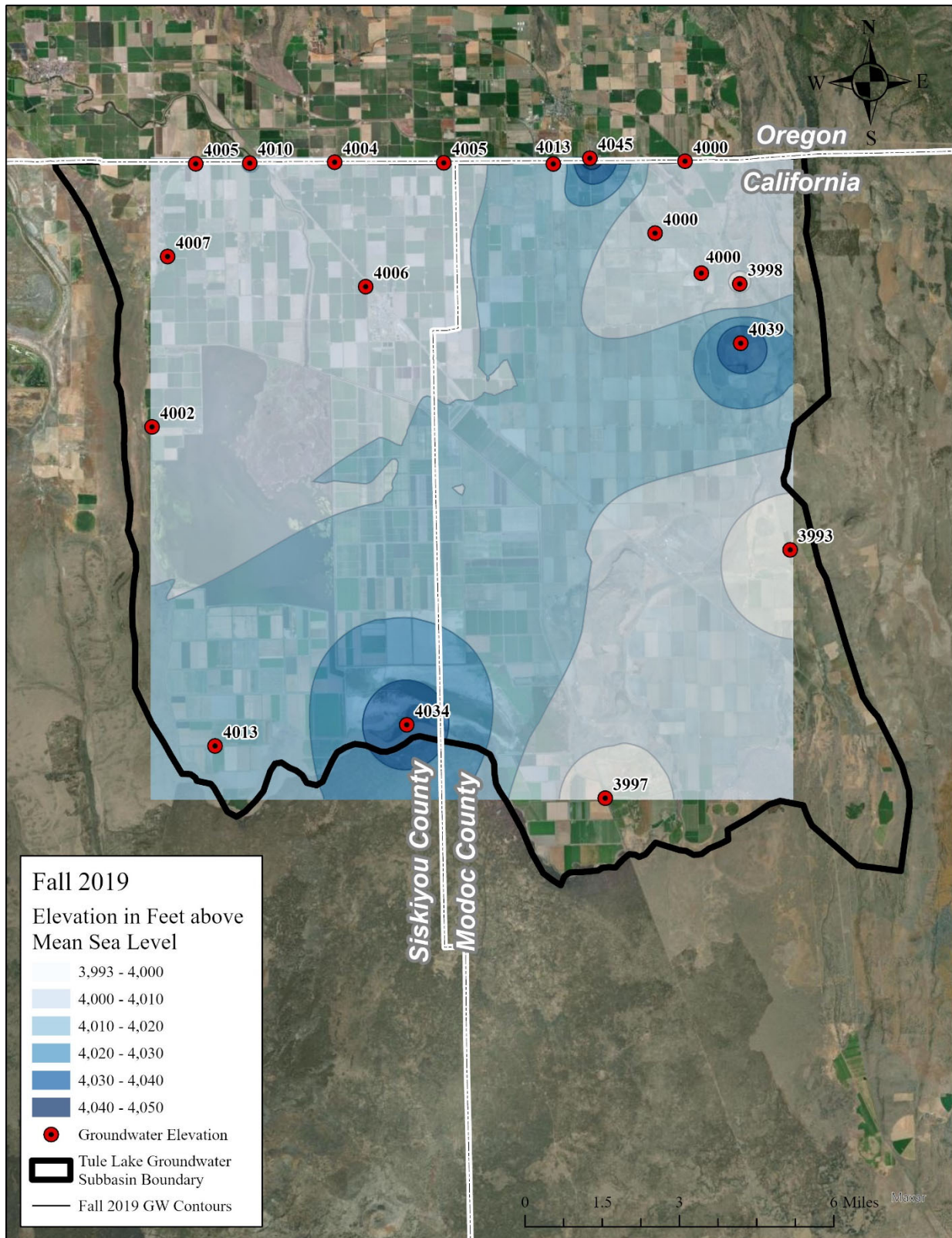
Figure 2-5. Fall 2019 Groundwater Surface Elevations
