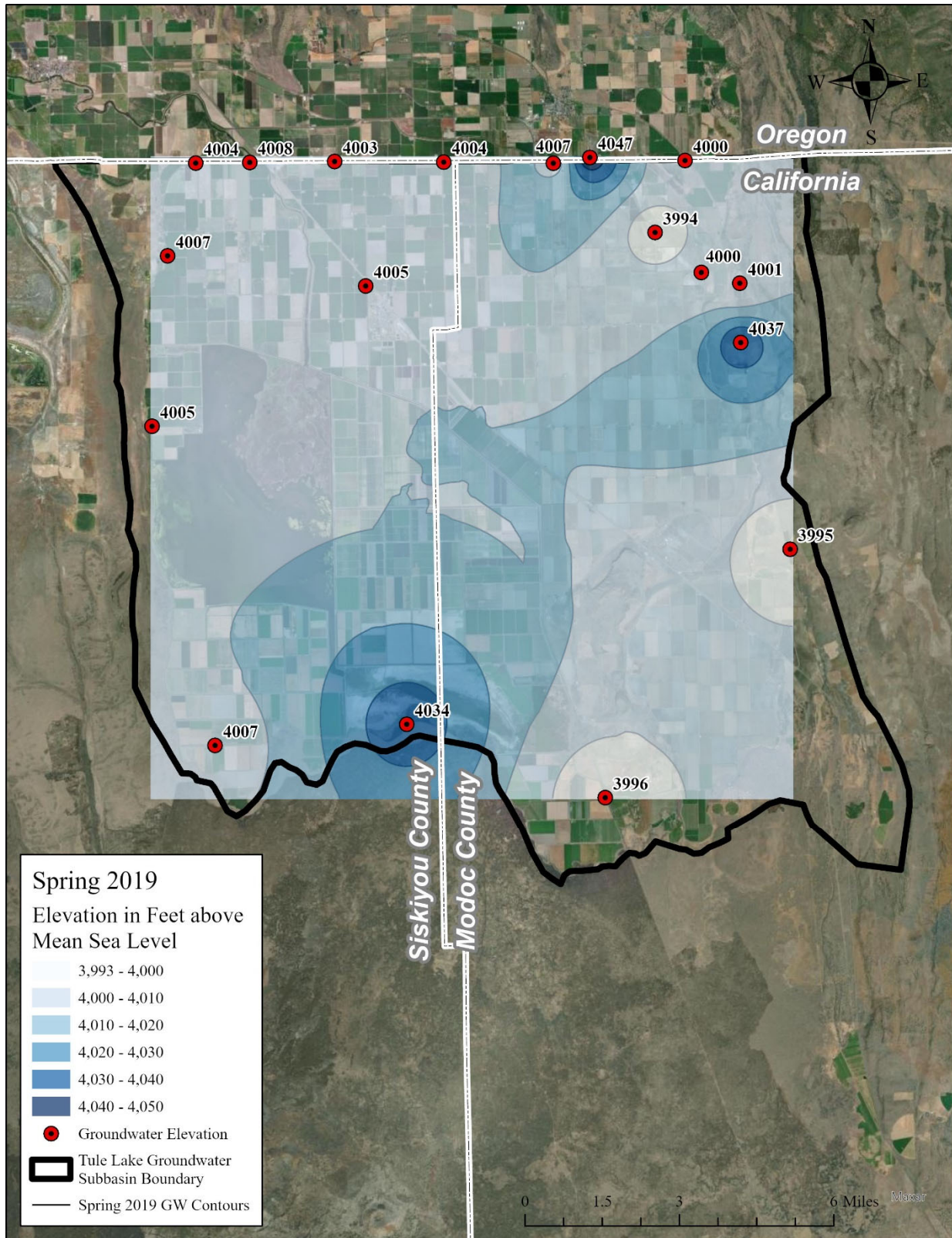
Figure 2-4. Spring 2019 Groundwater Surface Elevations
