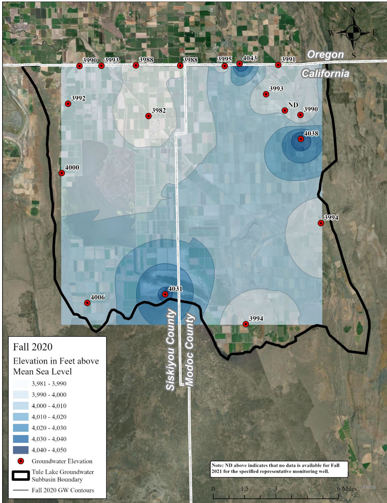
Figure 2-7. Fall 2020 Groundwater Surface Elevations
