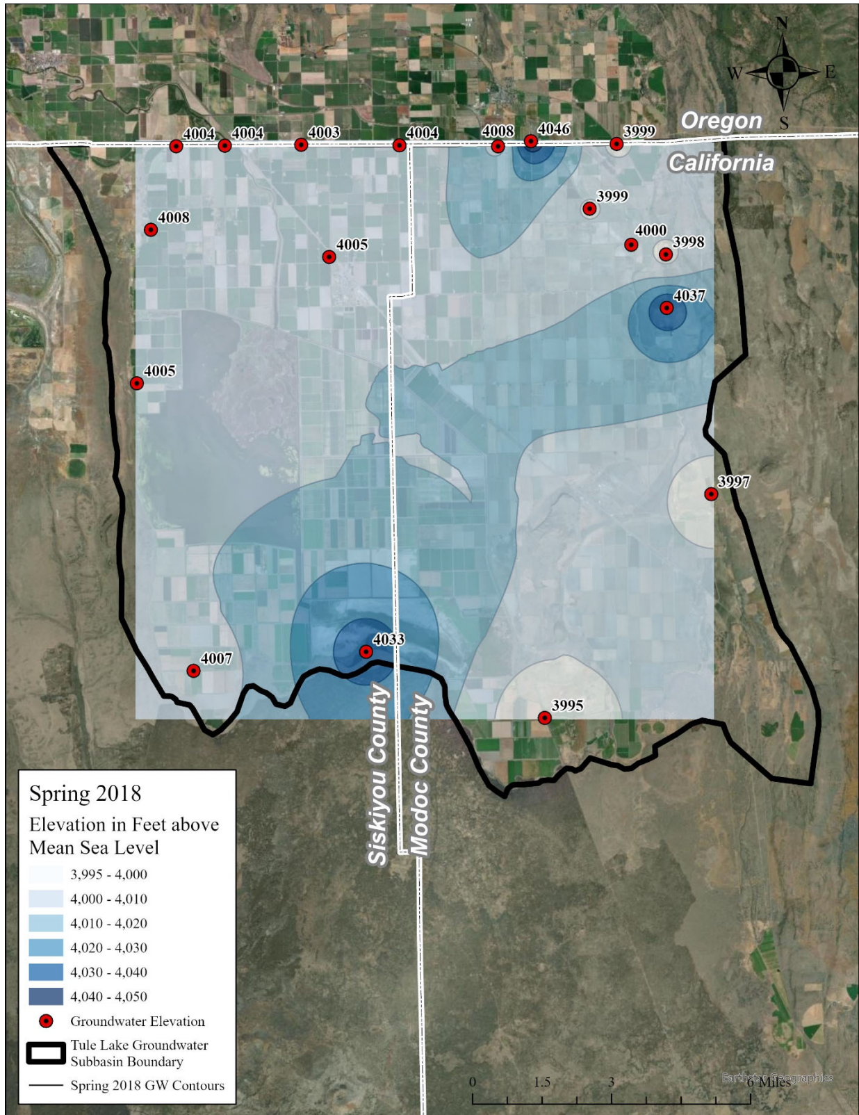
Figure 2-1. Spring 2018 Groundwater Surface Elevations
