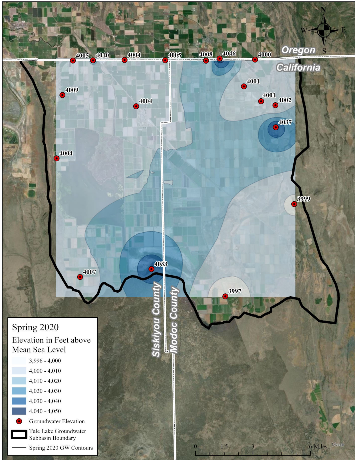
Figure 2-6. Spring 2020 Groundwater Surface Elevations
